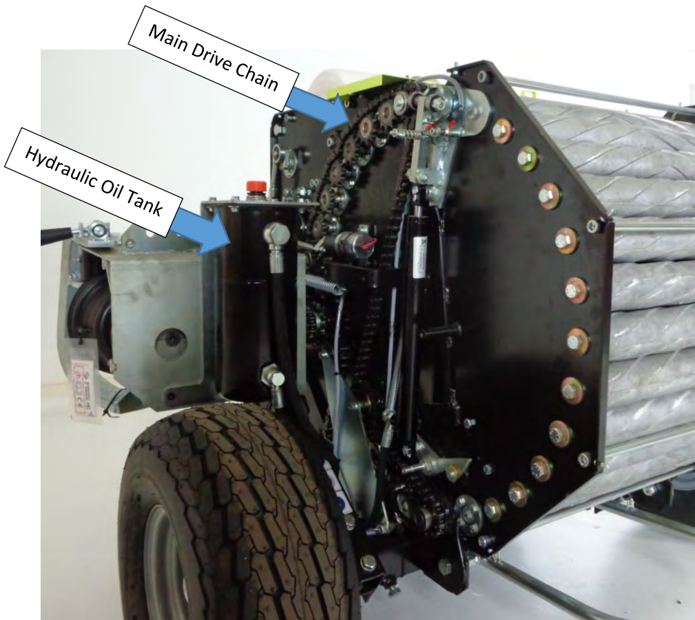
Figure 2 right side of baler with covers removed
